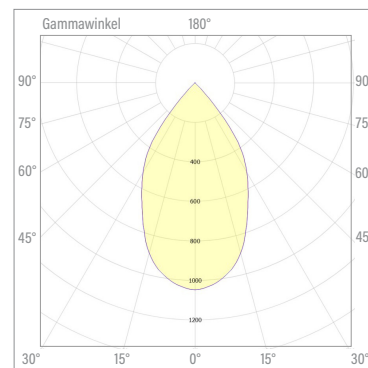
60° Wide Flood
